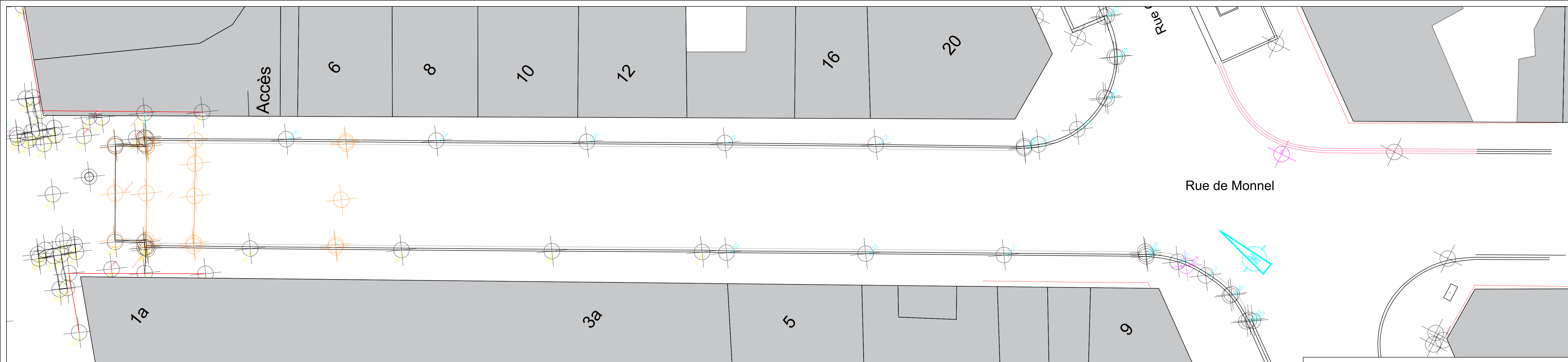
Plan terrier existant 1/100
